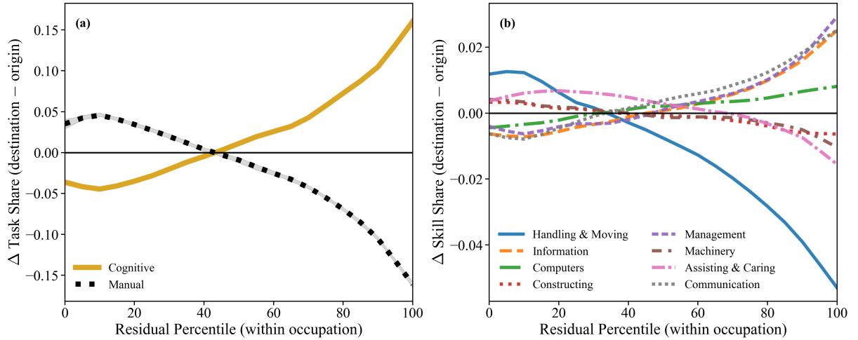
Figure 4: Panel (a): Change in cognitive and manual task shares (vertical axis) by residualized within-occupation wage percentile (horizontal axis) for occupational movers. Change is \Delta \text{Task-Share}_p^k = \text{LOWESS}_p(\omega_{j'(i)}^k - \omega_{j(i)}^k) , the smoothed difference in task intensities between destination j'(i) and origin j(i) occupations. Panel (b): Analogous changes based on the ESCO skill classification. By construction, given that \sum_k \omega_j^k = 1 , the non-parametric average shares per percentile sum up to 0.
