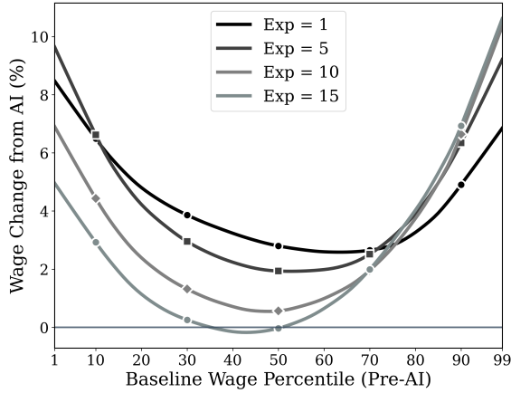
(a) Wage gains from AI by baseline wage percentile
