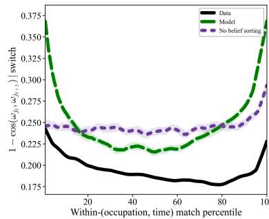
(b) Task distance of the switch
