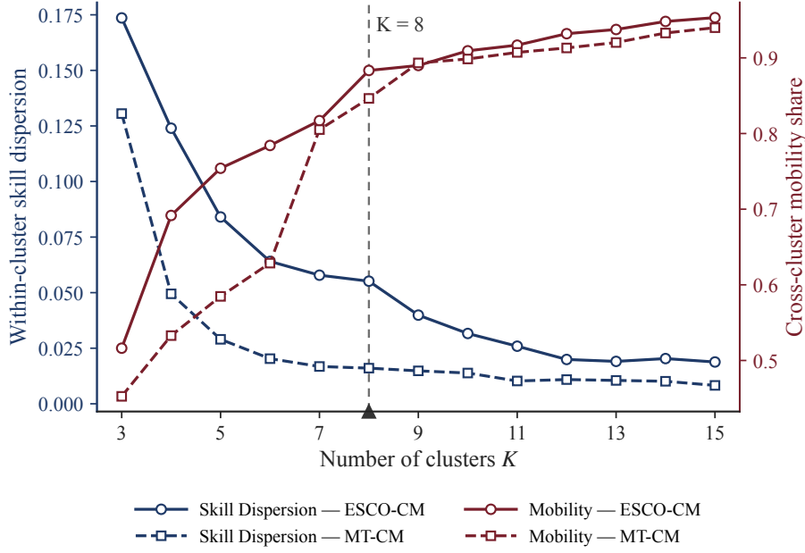
Figure 30: Headline diagnostic for the K -selection step of the anchored skill+mobility-penalty clustering. The horizontal axis is the number of clusters K on the 3–15 grid (with \lambda_{\text{user}} = 10 fixed at the empirical knee). Curves report the \omega -weighted within-cluster skill dispersion and the cross-cluster mobility share at the L -minimizing partition, separately for the ESCO-based cognitive/manual shares ( C_i, M_i ) and the task-based cognitive/manual shares ( C_i^{\text{MT}}, M_i^{\text{MT}} ), in both cases with the cognitive anchor \{241, 412, 431\} and the manual anchor pinned. The chosen K = 8 sits inside the dispersion plateau and one notch below the feasibility ceiling under both feature sets.
